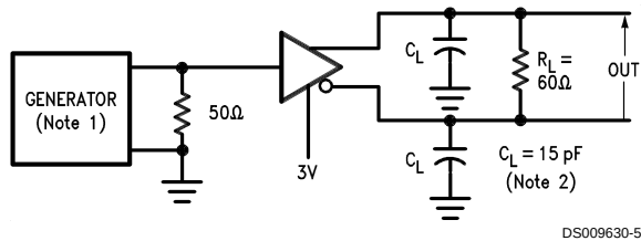
FIGURE 4. Driver Differential Output Delay and Transition Times
